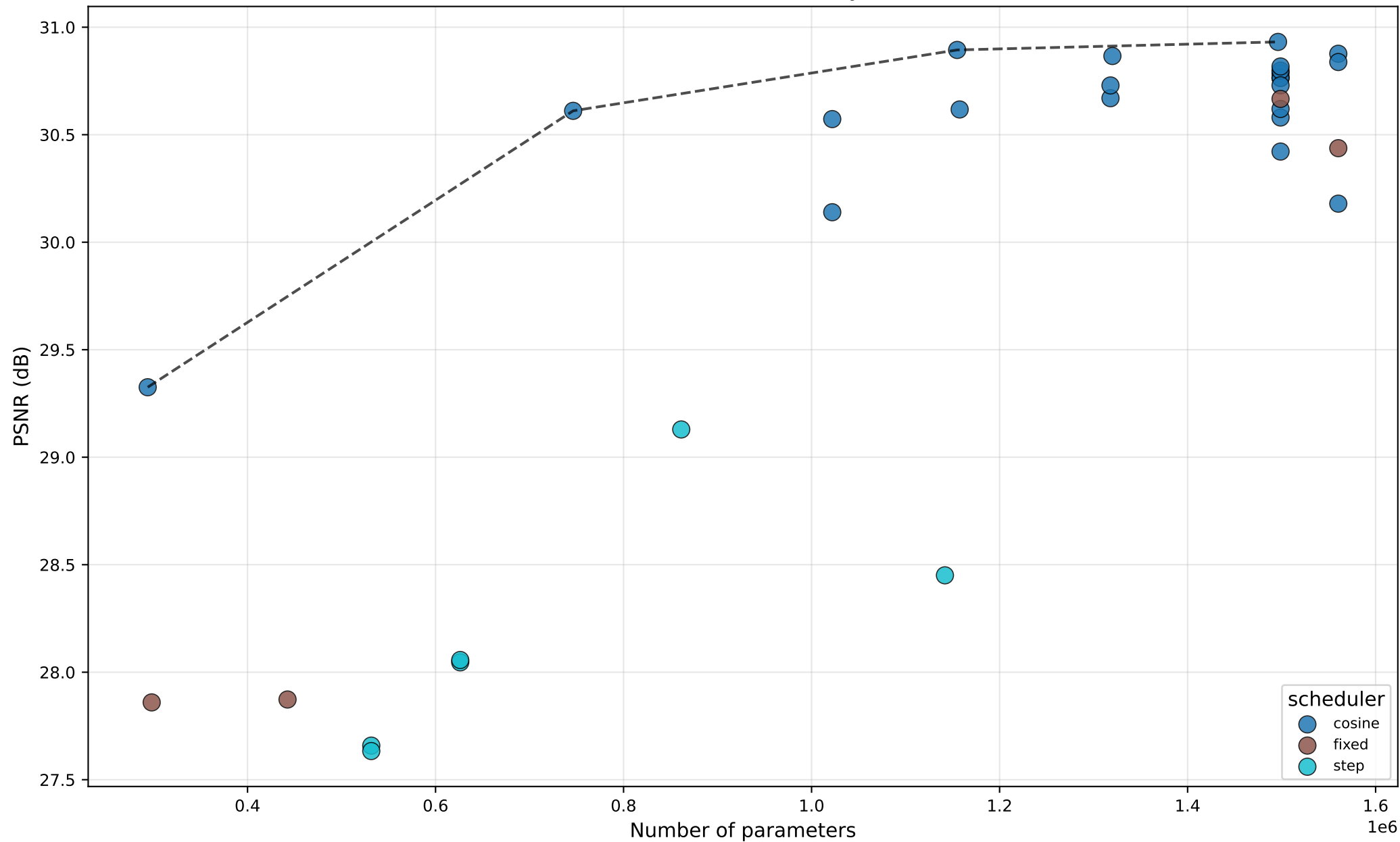
PSNR vs #Params — DAT — by scheduler
